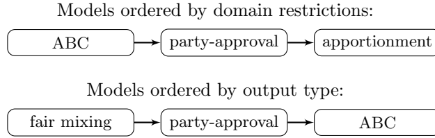
Figure 1: Relation of party-approval elections to other voting settings. An arrow from X to Y means that model X is more general than model Y . In the settings in the top row, elections return sets of alternatives but the models impose different restrictions on the input profiles: for ABC voting every input profile is allowed, for party-approval profiles each voter can for each party (viewed as a set of alternatives) either approve all of its members or none, and for apportionment each voter must approve all members of exactly one party. In the bottom row, the models are ordered with respect to their output type: all of fair mixing, party-approval elections, and ABC elections can take arbitrary approval profiles as input, but fair mixing rules return a probability distribution over the alternatives, party-approval rules choose a multiset of the alternatives, and ABC rules choose a subset of the alternatives. This shows that party-approval elections can be seen both as generalization and special case of ABC elections.
