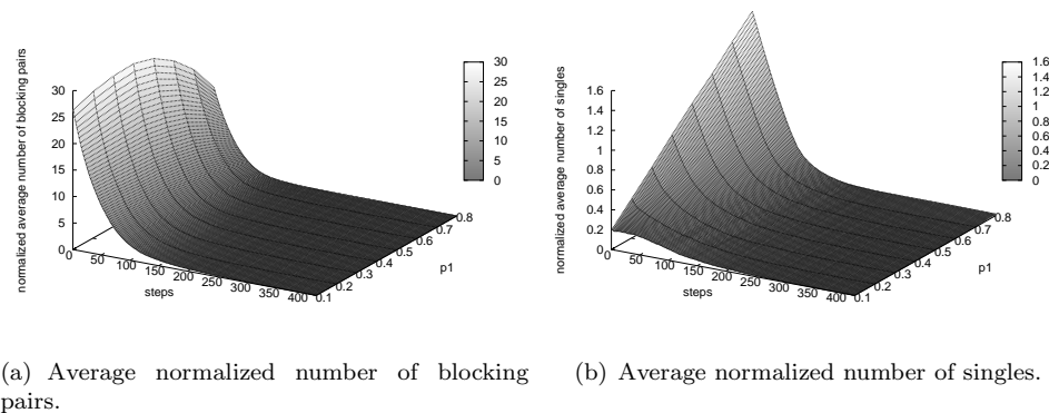
Figure 5: LTIU runtime behaviour ( p_2=0.5 ).
