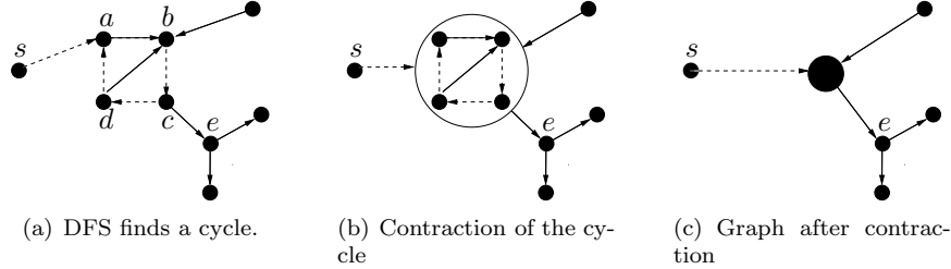
Figure 1: Contraction of a cycle to a supernode
