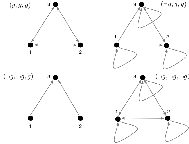
Figure 2: Some BR-dependences of Example 1.
