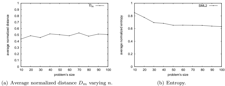
Figure 3: Sampling with SML2.
