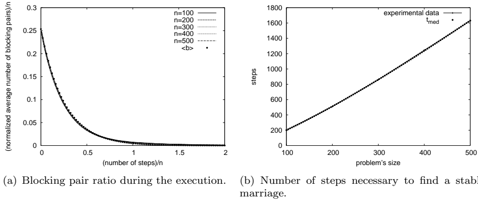
Figure 2: Results using SML2.
