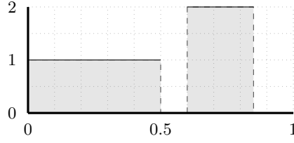
(a) Value density function for a piecewise constant valuation that is not piecewise uniform.
