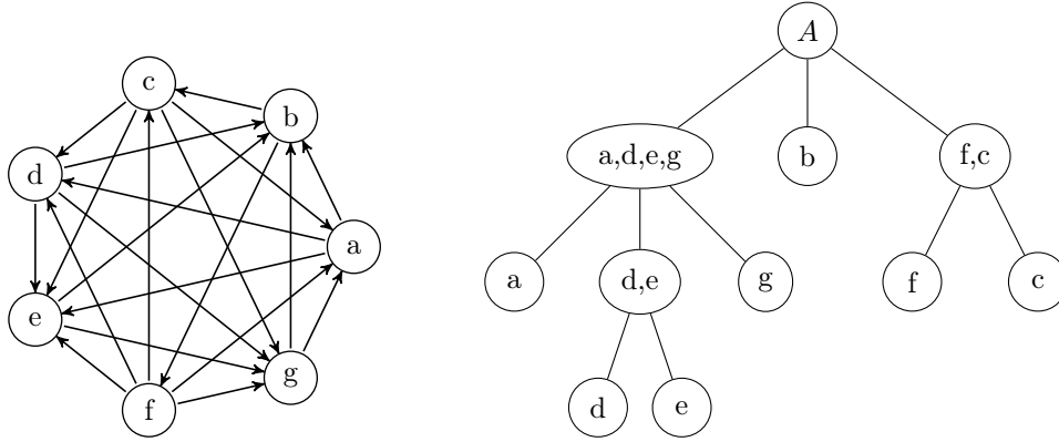
Figure 1: Example tournament with corresponding decomposition tree. Nodes \{f, c\} and \{d, e\} are reducible, all other nodes are irreducible. Curly braces are omitted to improve readability.
